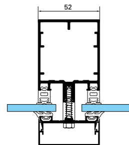
GEODE SG vidrio simple trama vertical
